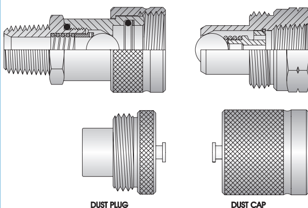
DUST PLUG
