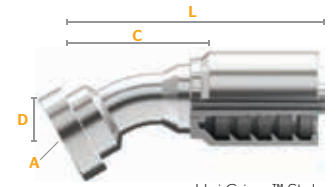
Uni-Crimp™ Style
