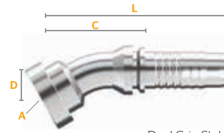
Dual-Grip Style
