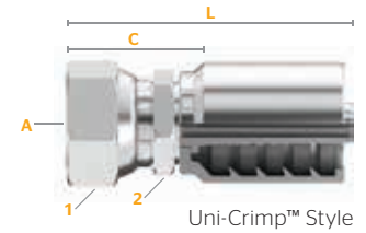
Uni-Crimp™ Style
