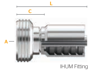
IHUM Fitting
