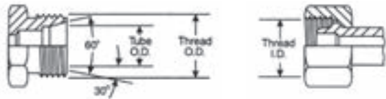
Male 60° Cone
