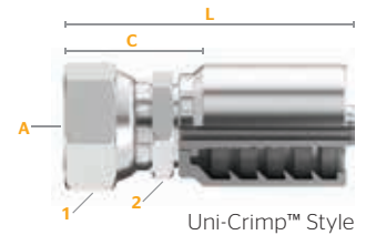
Uni-Crimp™ Style
